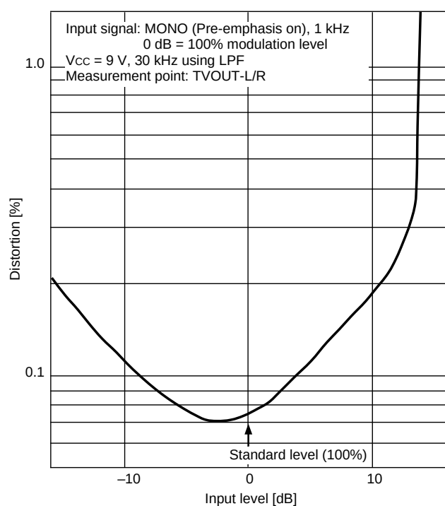
Input level vs. Distortion characteristics 1 (MONO)
