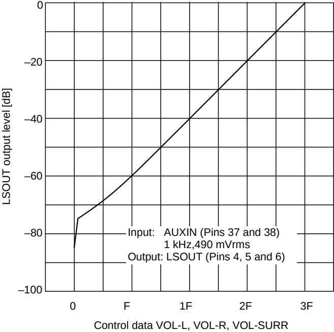
Volume characteristics
