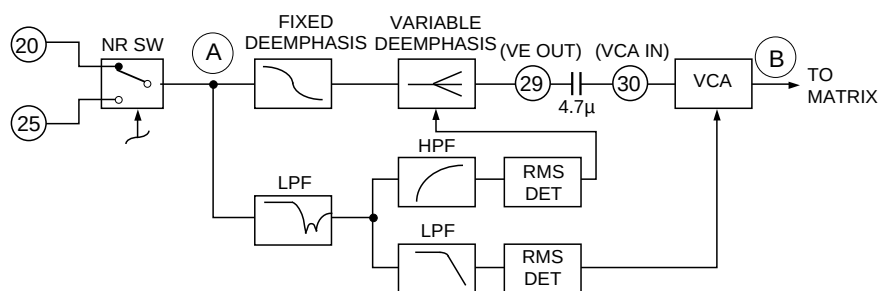
Fig 3. dbx-TV block
