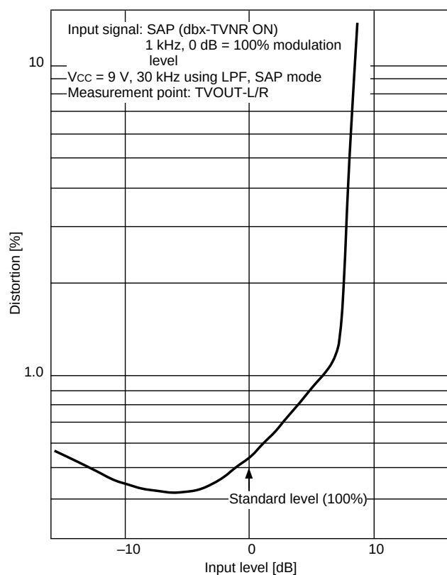
Input level vs. Distortion characteristics 3 (SAP)
