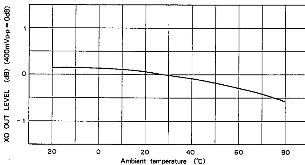
XO OUT LEVEL temperature characteristics
