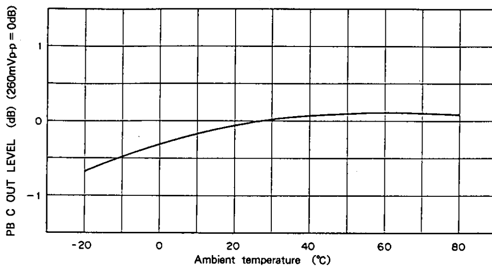
PB C OUT LEVEL temperature characteristics
