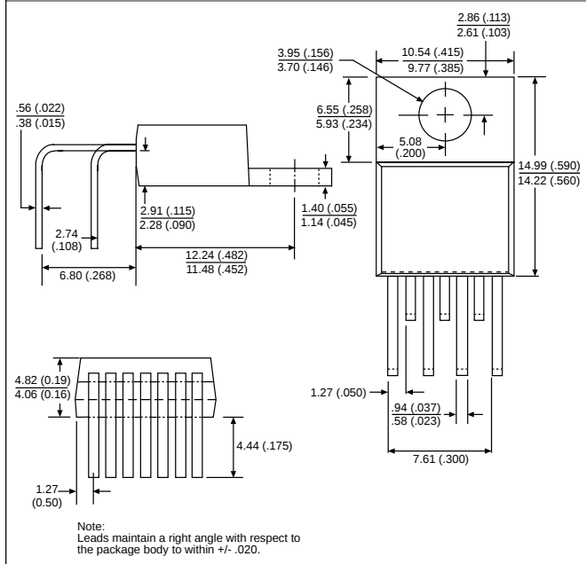
7 Lead TO-220 (THA) Horizontal
