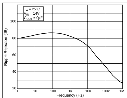
Regulator 2 Ripple Rejection
