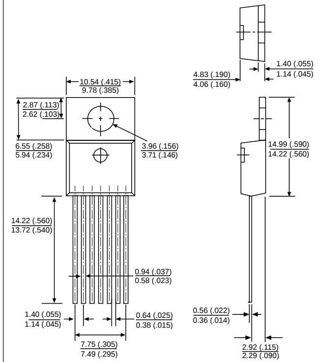
7 Lead TO-220 (T) Straight
