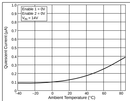
Quiescent Current
