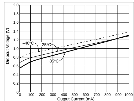
Regulator 1 Dropout Voltage
