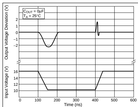
Regulator 1 Line Transient Response
