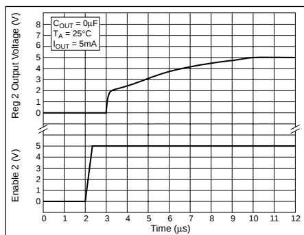
Regulator 2 Startup
