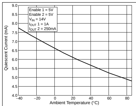
Quiescent Current
