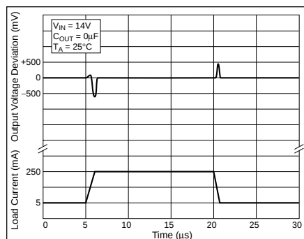
Regulator 2 Load Transient Response
