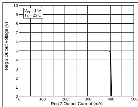
Regulator 2 Current Limit
