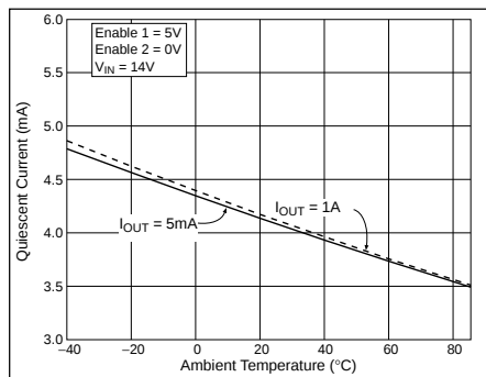
Regulator 1 Quiescent Current
