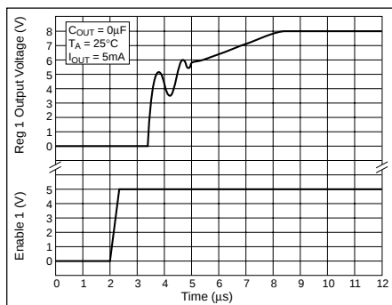
Regulator 1 Startup
