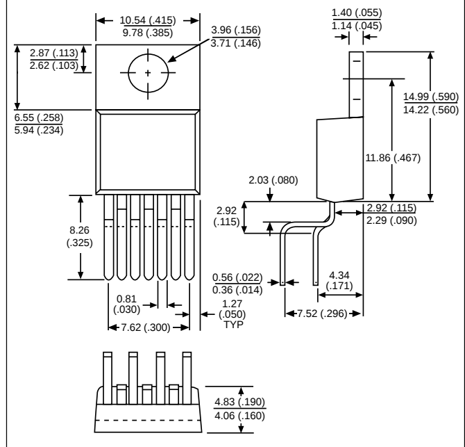
7 Lead TO-220 (TVA) Vertical
