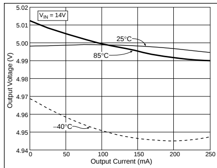
Regulator 2 Load Regulation
