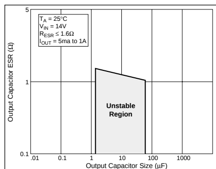
Regulator 1 Stability
