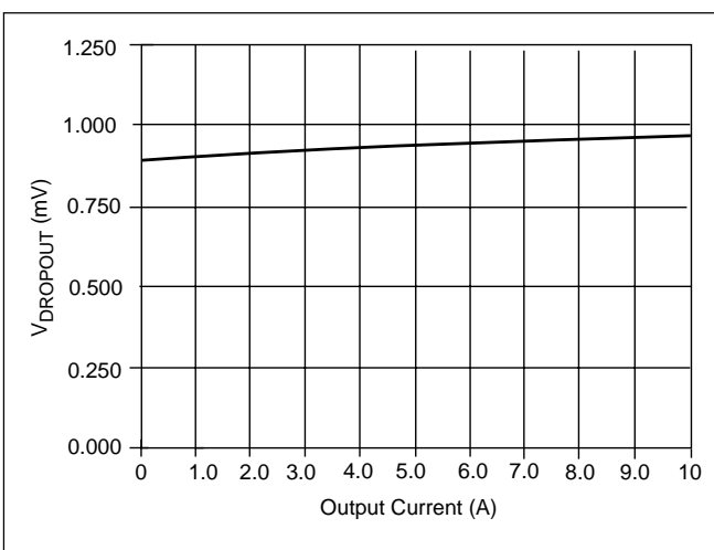
V_{\text{DROPOUT}} vs I_{\text{OUT}}
