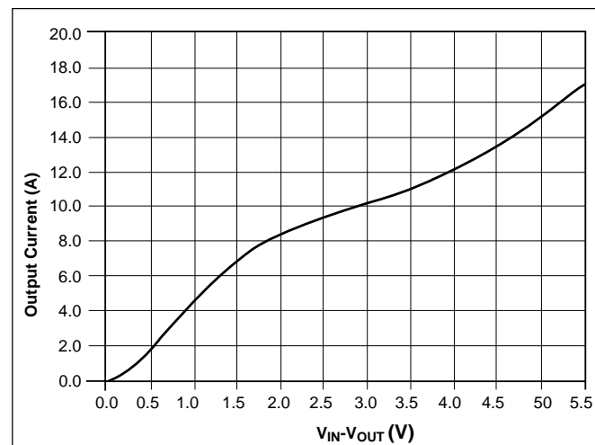
I_{\text{min}} vs V_{IN} - V_{OUT}
