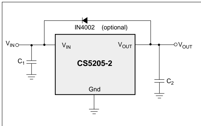
Figure 1. Protection diode scheme for fixed output regulators.
