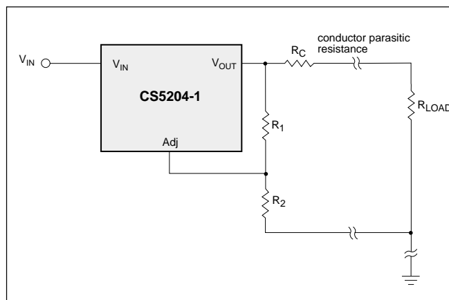
Figure 4. Grounding scheme for the adjustable output regulator to minimize parasitics.
