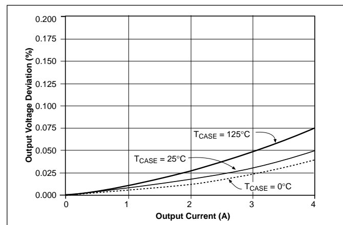
Load Regulation vs. Output Current
