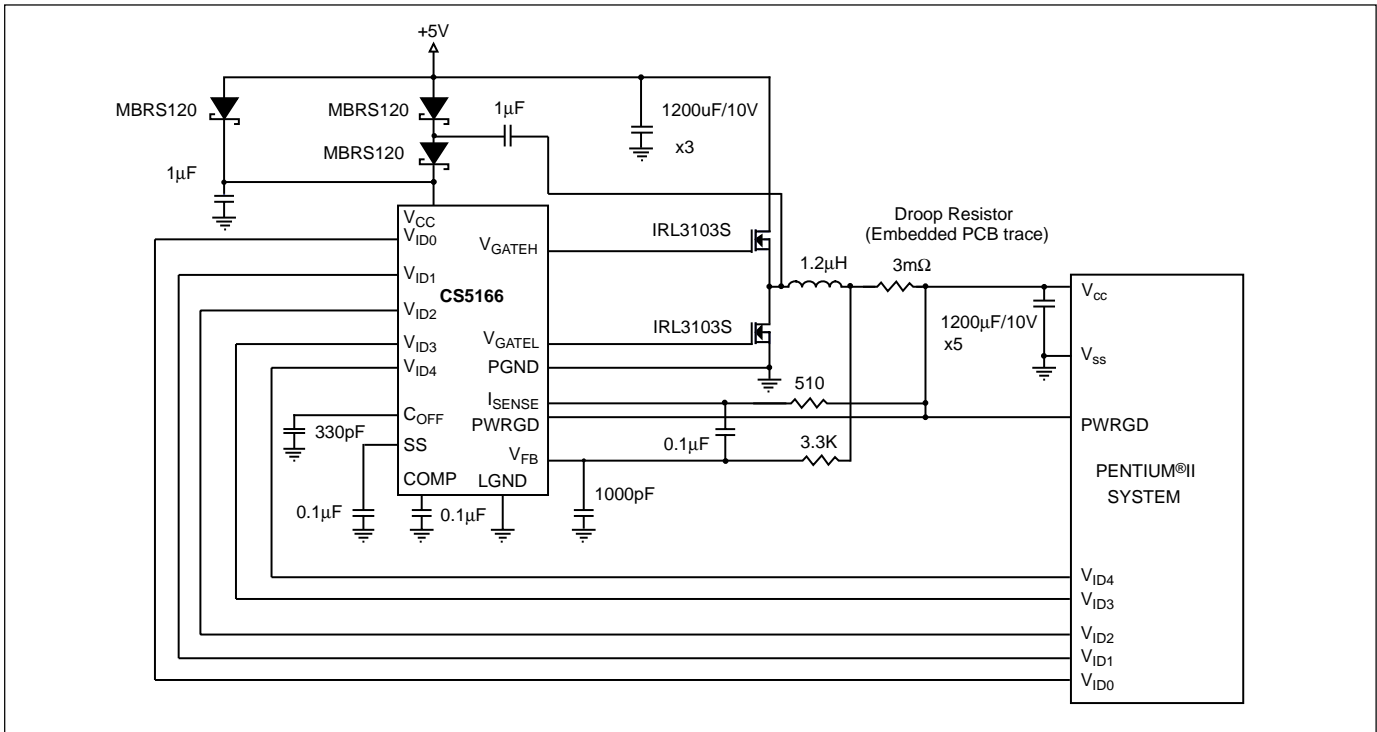
Figure 35: +5V to +2.8V @ 14.2A for 300 MHz Pentium® II.
