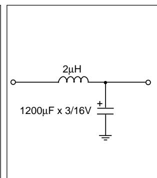
Figure 28: Input Filter.
