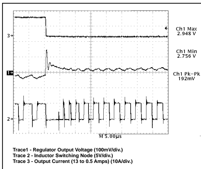
Figure 9: CS5158 demonstration board response to 13A load turn off (output set for 2.8V). V^{2TM} control topology immediately connects inductor to ground, providing 0% duty cycle. Regulation is achieved in less than 10μs.
