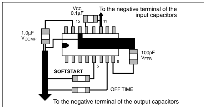
Figure 20: Layout Guidelines
