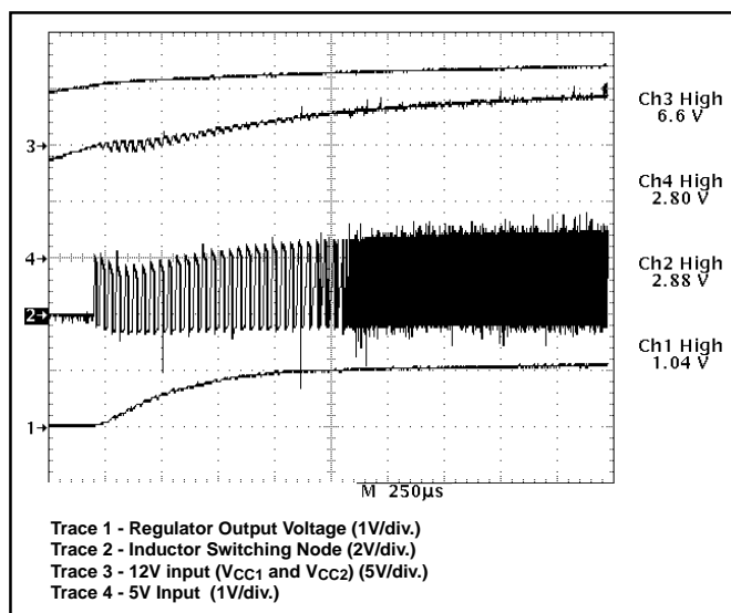
Figure 2: CS5157 demonstration board startup in response to increasing 12V and 5V input voltages. Extended off time is followed by normal off time operation when output voltage achieves regulation to the error amplifier output.
