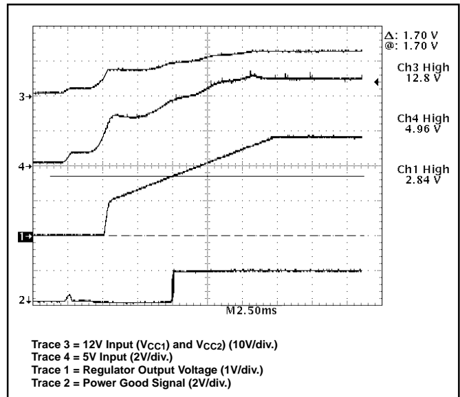
Figure 14: CS5156H demonstration board during power up. Power Good signal is activated when output voltage reaches 1.70V.
