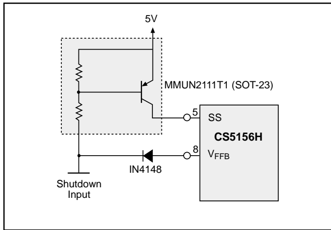
Figure 12: Implementing shutdown with the CS5156H.
