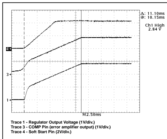
Figure 3: CS5156H demonstration board startup waveforms.
