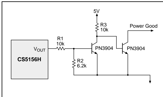
Figure 13: Implementing Power Good with the CS5156H.
