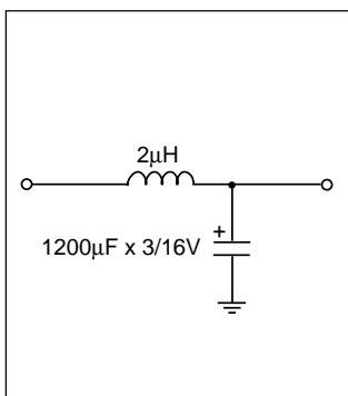
Figure 17: Input Filter
