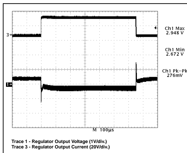
Figure 7: CS5156H demonstration board response to a 0.5 to 13A load pulse (output set for 2.8V).
