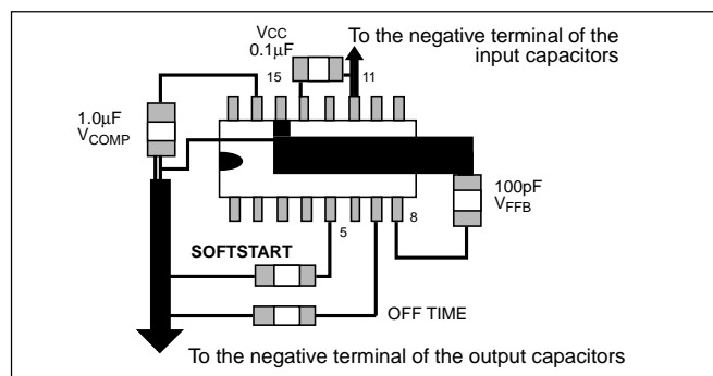
Figure 18: Layout Guidelines
