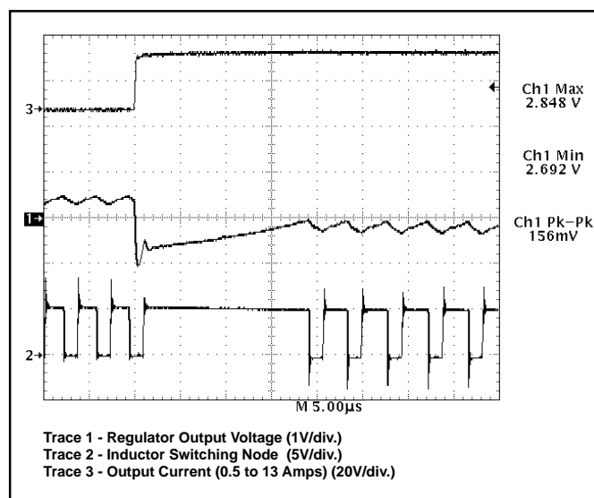
Figure 8: CS5156H demonstration board response to 13A load turn on (output set for 2.8V). Upon completing a normal off time, the V^{2TM} control loop immediately connects the inductor to the input voltage, providing 100% duty cycle. Regulation is achieved in less than 20μs.
