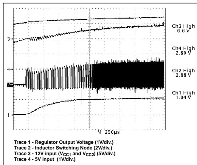
Figure 2: CS5156H demonstration board startup in response to increasing 12V and 5V input voltages. Extended off time is followed by normal off time operation when output voltage achieves regulation to the error amplifier output.
