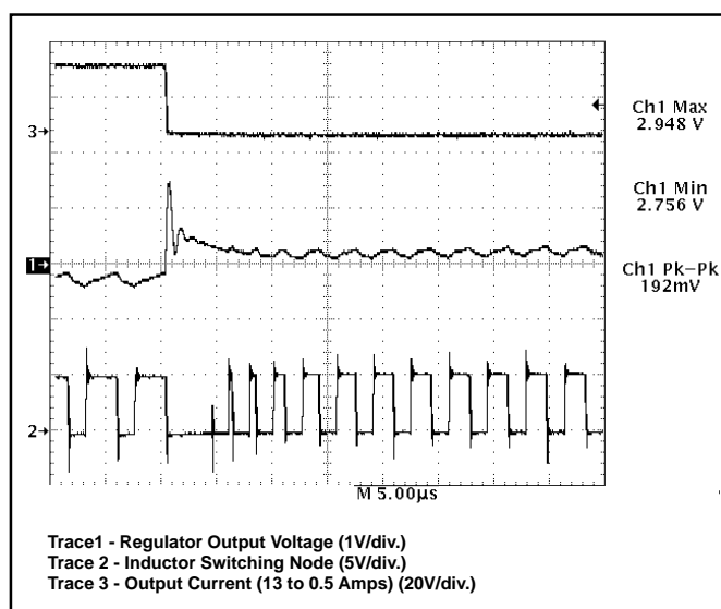
Figure 9: CS5156H demonstration board response to 13A load turn off (output set for 2.8V). V^2 ™ control topology immediately connects inductor to ground, providing 0% duty cycle. Regulation is achieved in less than 10µs.
