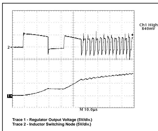
Figure 4: CS5156H demonstration board enable startup waveforms.
