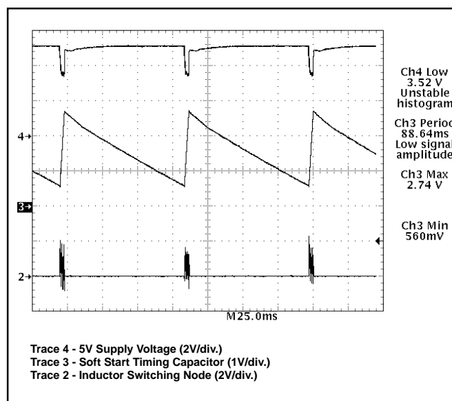
Figure 10: CS5156H demonstration board hiccup mode short circuit protection. Gate pulses are delivered while the soft start capacitor charges, and cease during discharge.
