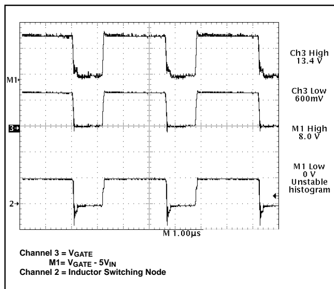
Figure 15: CS5156H gate drive waveforms depicting rail to rail swing.
