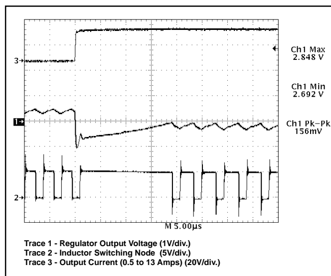
Figure 8: CS5156 demonstration board response to 13A load turn on (output set for 2.8V). Upon completing a normal off time, the V^2 ™ control loop immediately connects the inductor to the input voltage, providing 100% duty cycle. Regulation is achieved in less than 20μs.
