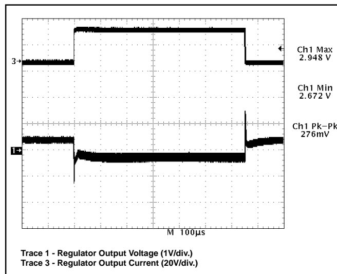
Figure 7: CS5155H demonstration board response to a 0.5 to 13A load pulse (output set for 2.8V).
