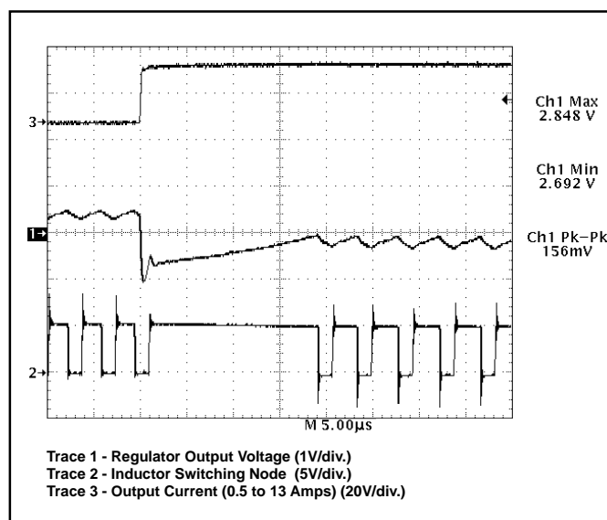
Figure 8: CS5150H demonstration board response to 13A load turn on (output set for 2.8V). Upon completing a normal off time, the V^2 ™ control loop immediately connects the inductor to the input voltage, providing 100% duty cycle. Regulation is achieved in less than 20μs.
