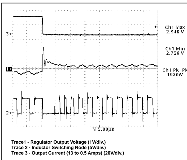
Figure 9: CS5150H demonstration board response to 13A load turn off (output set for 2.8V). V^2 ™ control topology immediately connects inductor to ground, providing 0% duty cycle. Regulation is achieved in less than 10μs.
