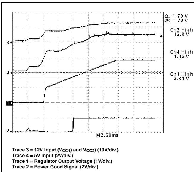
Figure 16: CS5150H demonstration board during power up. Power Good signal is activated when output voltage reaches 1.70V.
