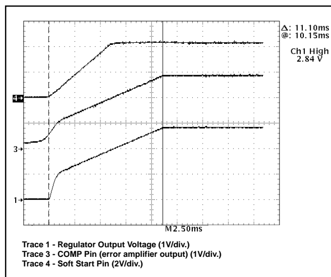
Figure 3: CS5150 demonstration board startup waveforms.
