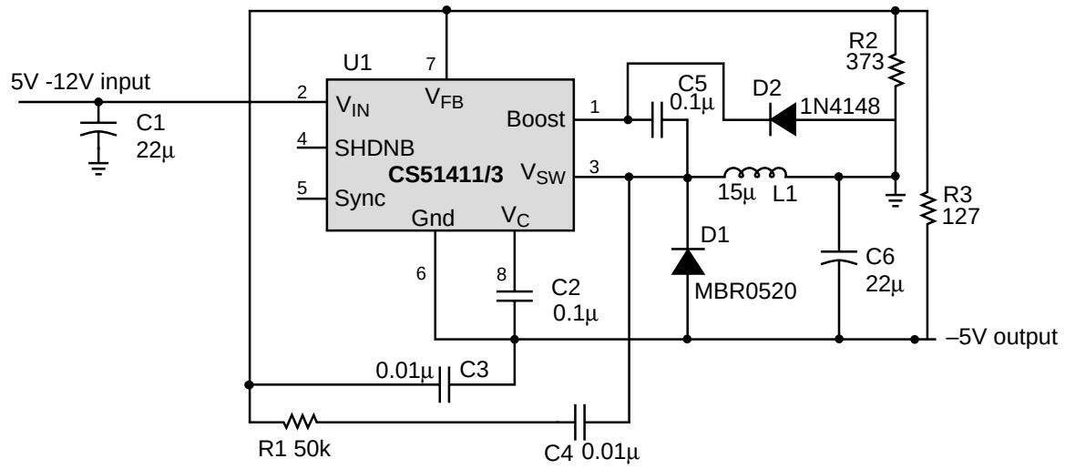
5V – 12V to –5V/400mA Inverting Converter
