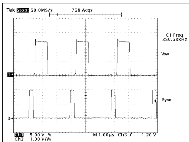
Figure 2: A CS51411 buck regulator is synced by an external 350kHz pulse signal.
