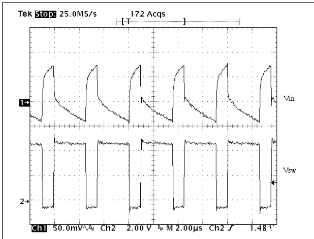
Figure 8: Input voltage ripple in a Buck converter.
