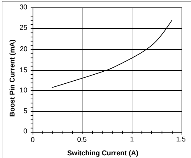
Figure 5: The boost pin current includes 7mA pre-driver current and base current when the switch is turned on. The beta decline of the power switch further increases the base current at high switching current.
