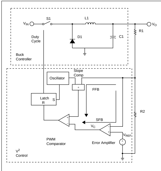
Figure 1: Buck converter with V 2 ™ control.
