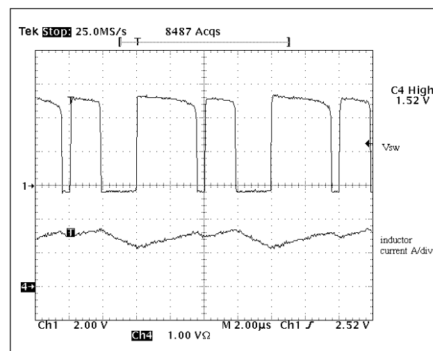
Figure 4: The regulator in current limit.
