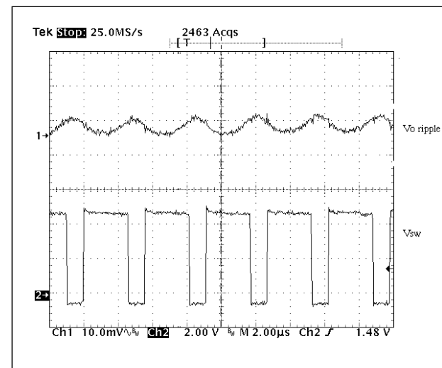
Figure 10: The output voltage ripple using two 10µF ceramic capacitors in parallel.
