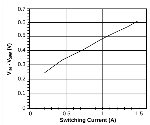
Figure 3: The saturation voltage of the power switch increases with the conducting current.
