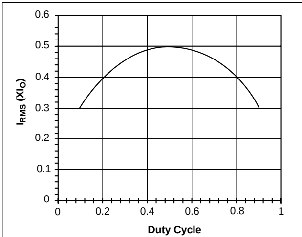
Figure 9: Input capacitor RMS current can be calculated by multiplying Y value with maximum load current at any duty cycle.
