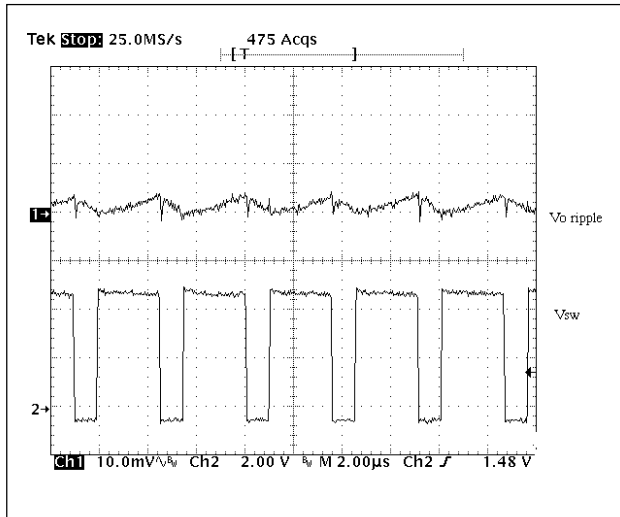
Figure 11: The output voltage ripple using one 100µF POSCAP capacitor.
