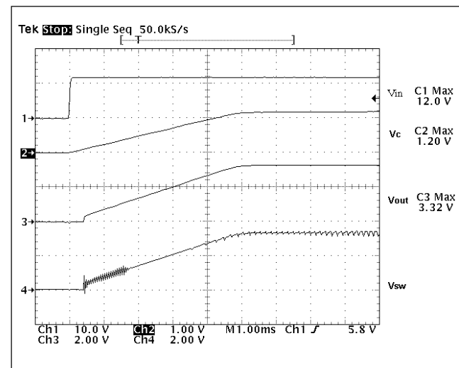
Figure 6: The power up transition of C5141X regulator.
