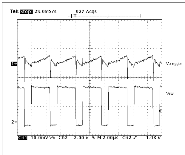
Figure 12: The output voltage ripple using one 100µF OS-CON
