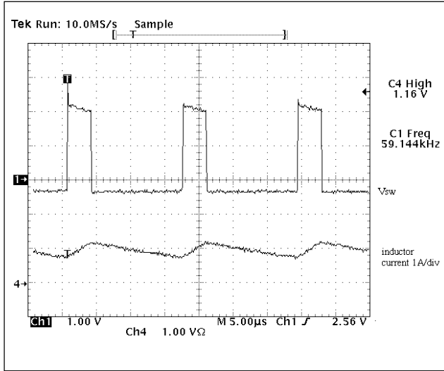
Figure 7: In short circuit, the foldback current and foldback frequency limit the switching current to protect the IC, inductor and catch diode.
