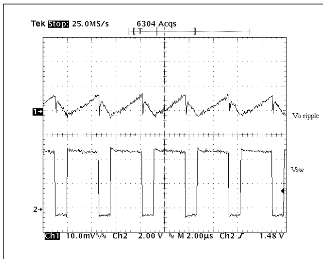
Figure 13: The output voltage ripple using one 100µF tantalum capacitor.
