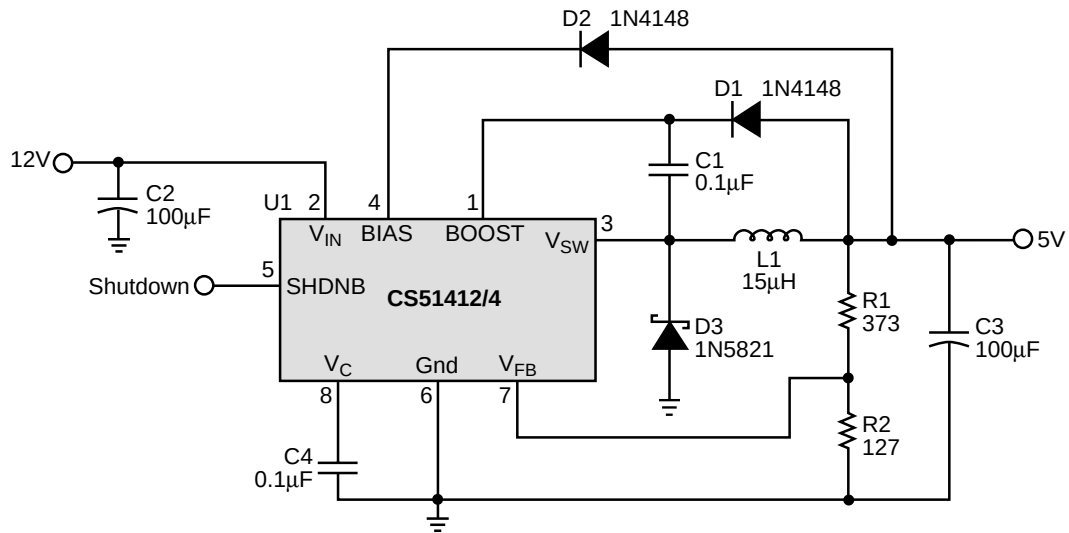
12V to 5V/1A Buck Converter using the BIAS pin.
