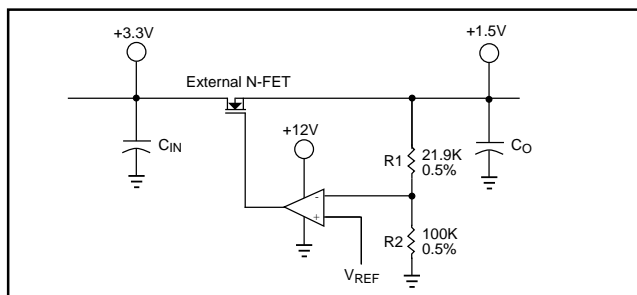
Figure 7: V_{REF} used in an N-FET LDO regulator.
