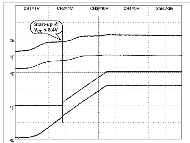
Figure 7: Normal Startup (2ms/div).
