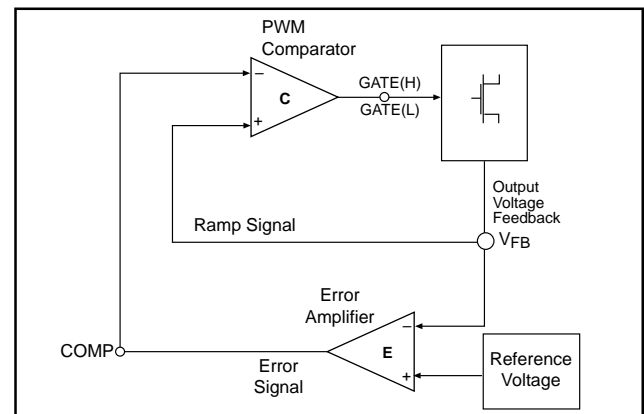
Figure 6: V^{2TM} Control Diagram
