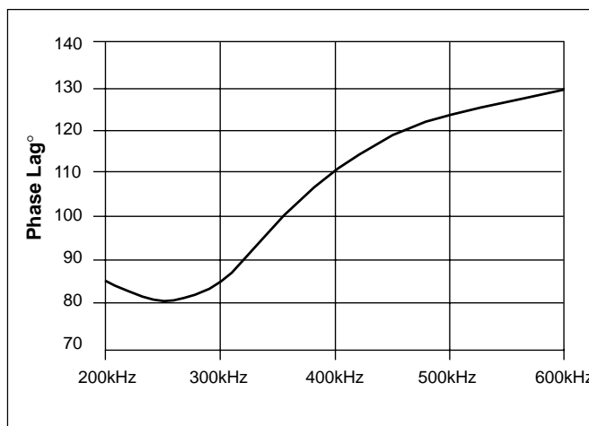
Figure 4: Typical Phase Lag between SYNC and GATE on.
