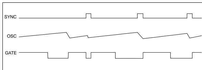
Figure 3. Synchronized Operation
