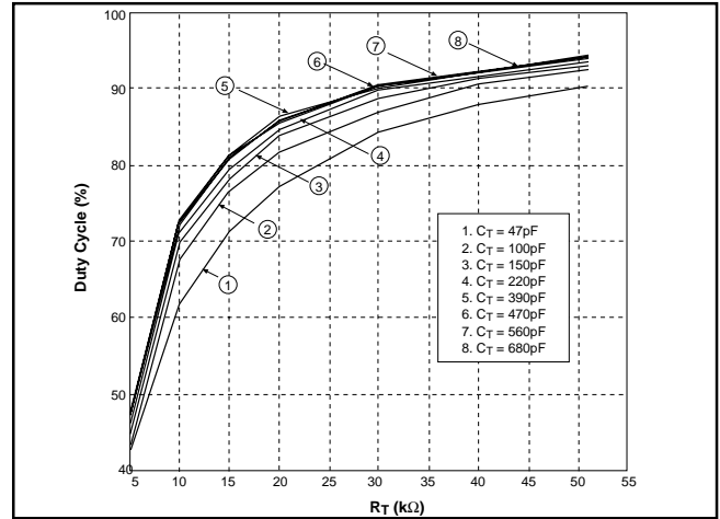
Figure 6: Duty Cycle vs. R_T for Discrete Capacitor Values.
