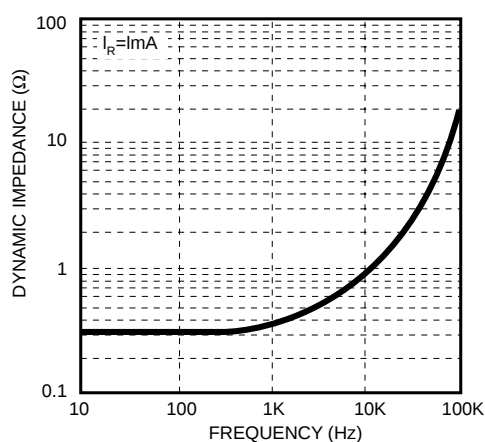
Dynamic Impedance vs. Frequency
