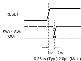
Fig. 8 Reset and output relationship (reset transmission time)
