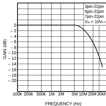
Fig. 13 Frequency characteristic(OUT1)
