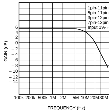
Fig. 15 Frequency characteristic (OUT2 and OUT3)
