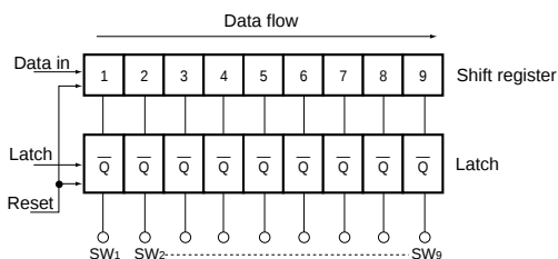
Fig. 5 Digital block
