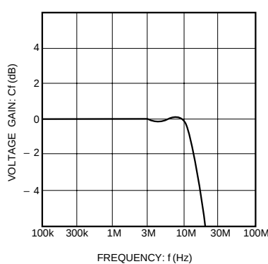
Fig. 3 Frequency characteristics
