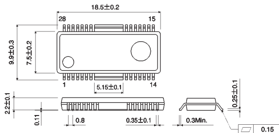
HSOP28
