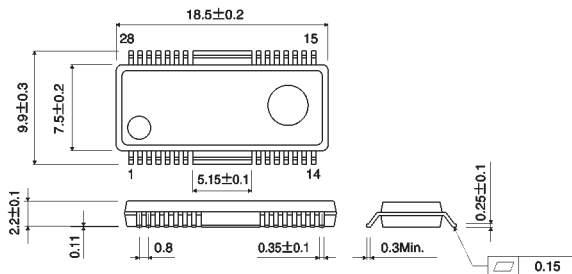
HSOP-M28
