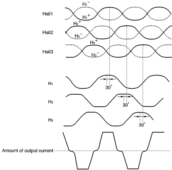
Fig.16 I/O waveforms
