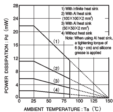
Fig.11 Thermal derating characteristics
