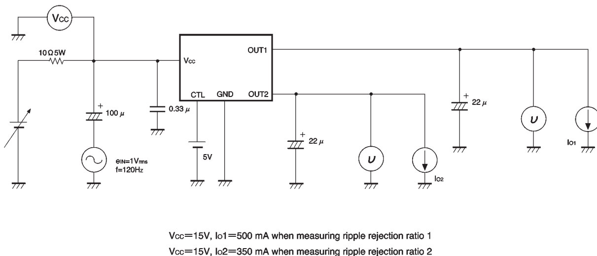
Fig.2 Circuit for measuring ripple rejection ratio
