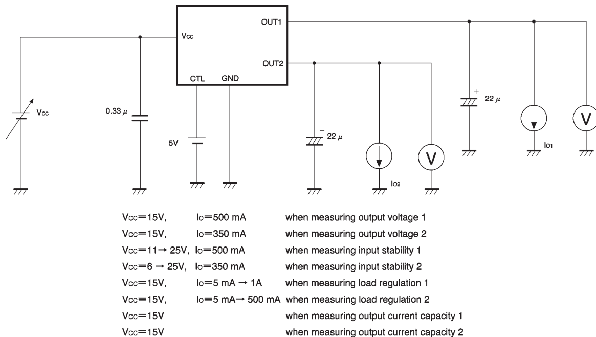
Fig.1 Circuit for measuring output voltage, input stability, load regulation, and output current capacity
