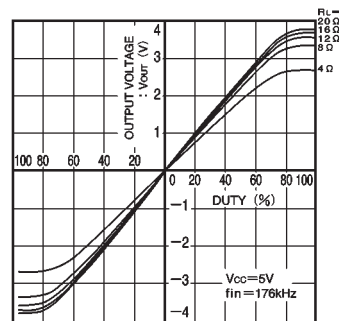
Fig. 9 Driver I/O characteristics (variable load)
