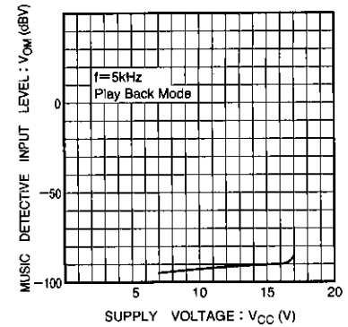
Fig. 19 Music detective input level vs. supply voltage
