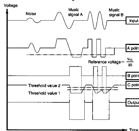
Fig. 4 Timing chart 1 (short time set for song gap detection)
