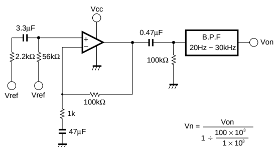
Fig. 8 Input conversion noise voltage
