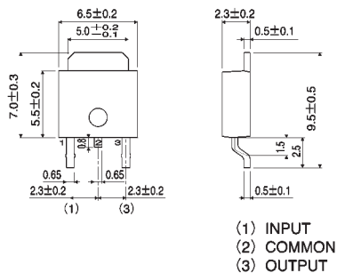
TO252-3
