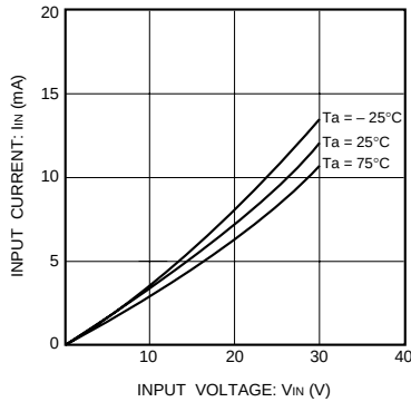
Fig. 17 Input current vs. input voltage (BA12003B / BF)
