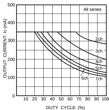
Fig. 9 Output conditions (I)
