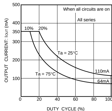
Fig. 10 Output conditions (II)
