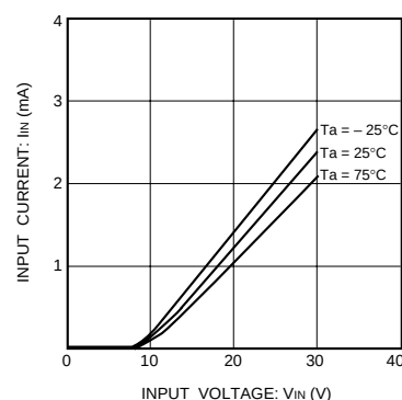
Fig. 16 Input current vs. input voltage (BA12002)
