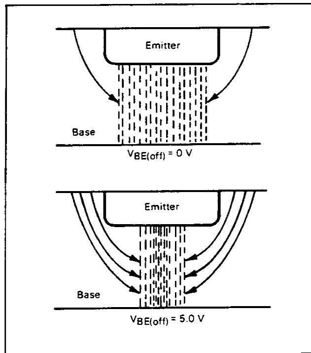
FIGURE 8 — RBSOA Current Crowding
