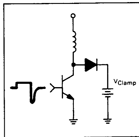
FIGURE 5 — RBSOA Test Circuit
