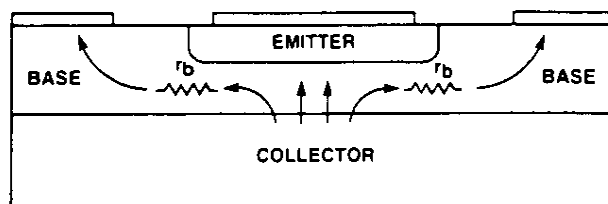
FIGURE 9 — Emitter Finger Crosssection
