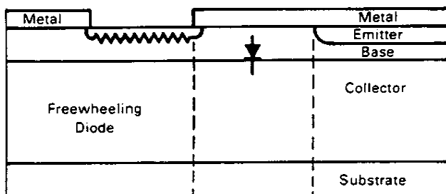
FIGURE 10 — Parasitic Freewheeling Diode
