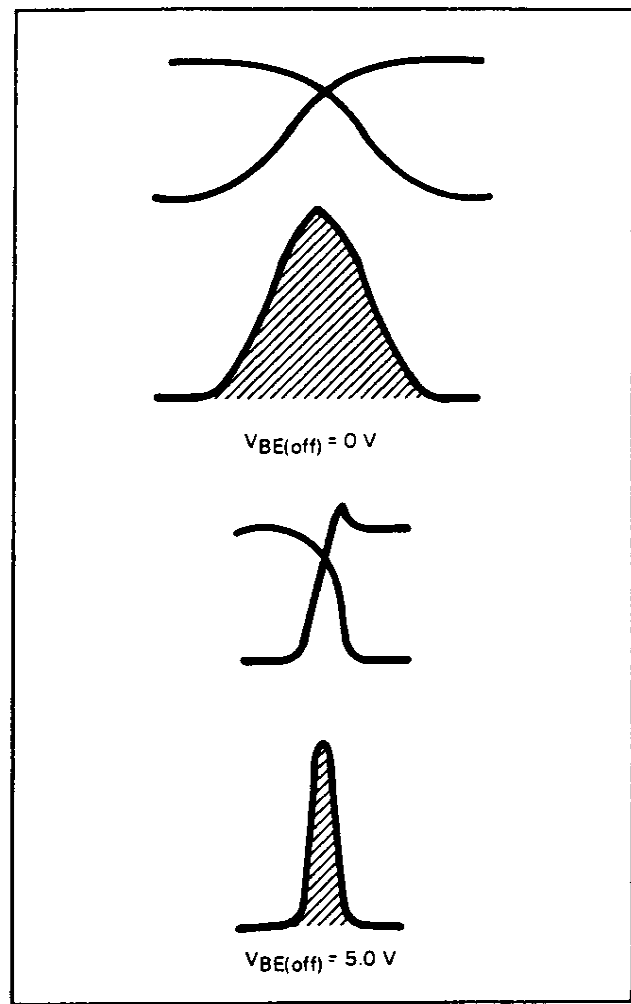
FIGURE 7 — RBSOA Energy Relationships
