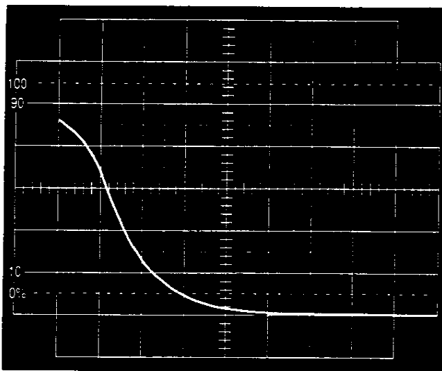
PHOTO 4 MOV (27 V) Vert: 10 V/div Horiz: 0.5 ms/div Transient Source Impedance: 50 \Omega V_{peak} = 44.7 V
