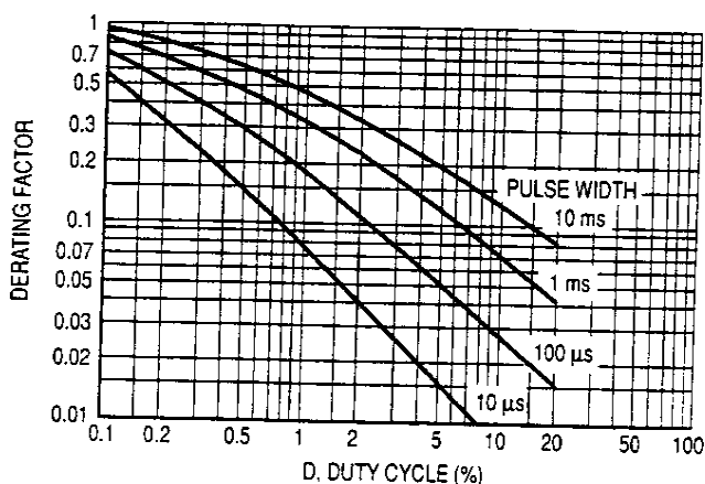
Figure 9. Typical Derating Factor for Duty Cycle
