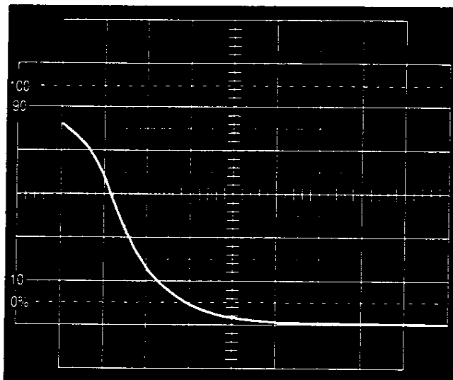
PHOTO 6 MOV (27 V) Vert: 10 V/div Horiz: 0.5 ms/div Transient Source Impedance: 5 \Omega V_{peak} = 52 V
