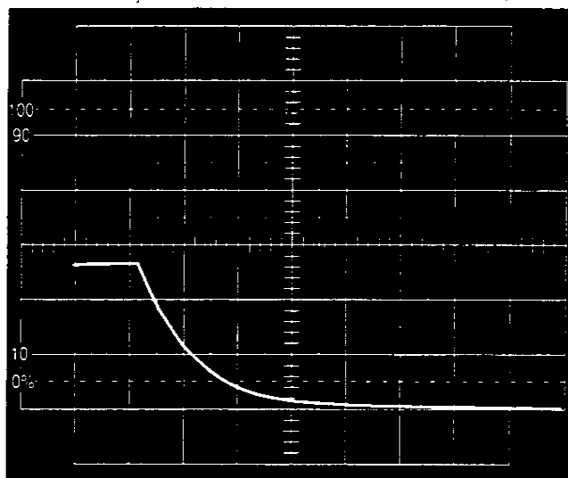
PHOTO 3 Zener (27 V) Vert: 10 V/div Horiz: 0.5 ms/div Transient Source Impedance: 500 \Omega V_{peak} = 27 \text{ V}
