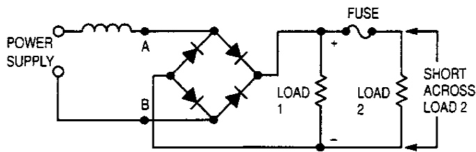
Figure 1. Load Dump with Inductive Power Supply
