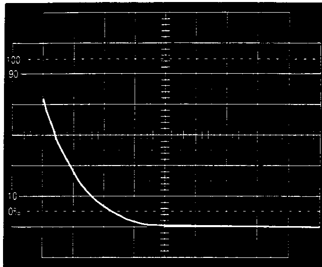
PHOTO 1 Open Circuit Transient Pulse Vert: 20 V/div Horiz: 0.5 ms/div V_{peak} = 90 \text{ V}
