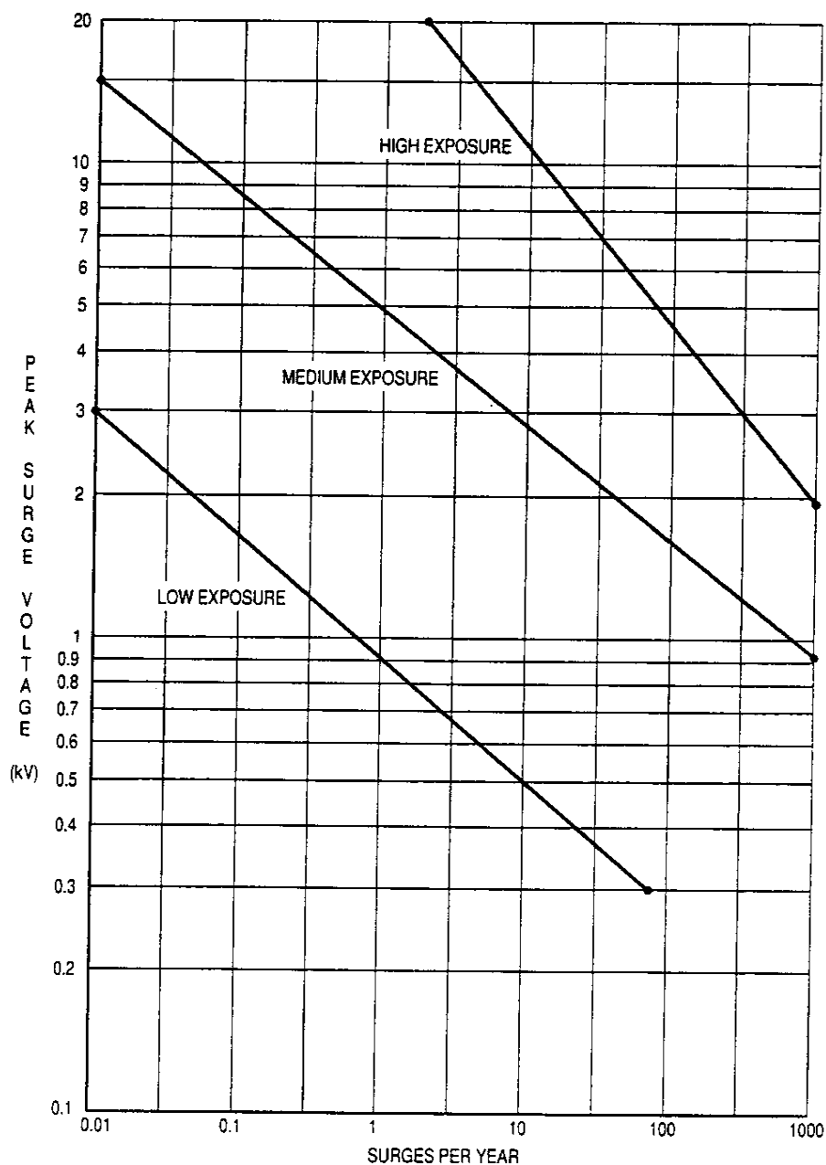
Figure 7. Peak Surge Voltage versus Surges per Year*
