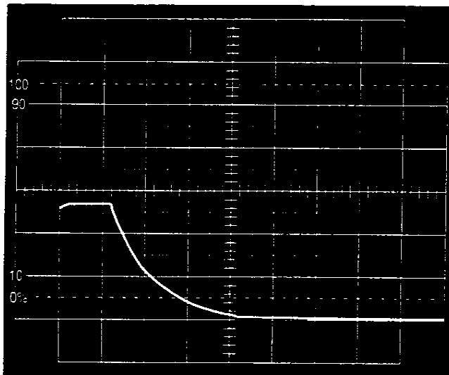
PHOTO 5 Zener (27 V) Vert: 10 V/div Horiz: 0.5 ms/div Transient Source Impedance: 50 \Omega V_{peak} = 27 V
