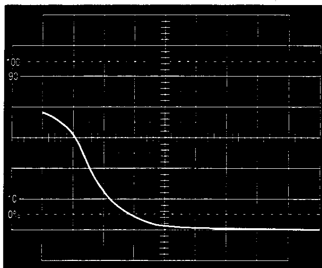
PHOTO 2 MOV (27 V) Vert: 10 V/div Horiz: 0.5 ms/div Transient Source Impedance: 500 \Omega V_{peak} = 39.9 \text{ V}
