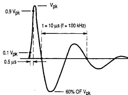
Figure 5. 0.5 ms 100 kHz Ring Wave
