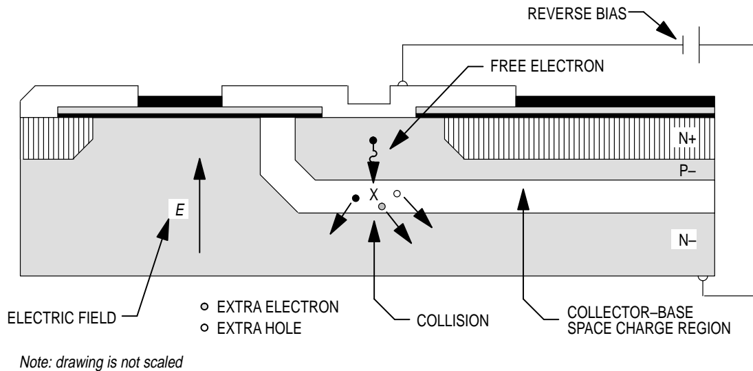
Figure 1. Simplified Representation of the Avalanche Process in a Junction
