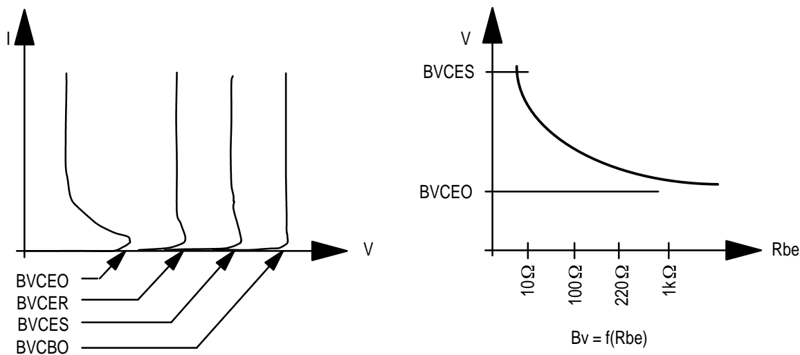
Figure 14. Typical Breakdown Curves (BVEBO not shown)
