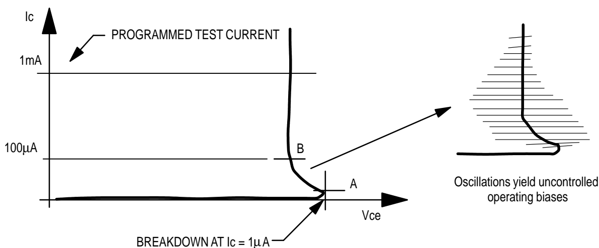
Figure 13. Typical BVCEO Characteristic
