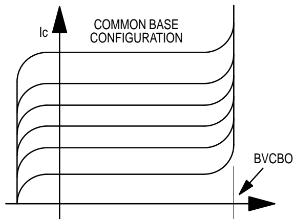
Figure 3a: Under breakdown, the emitter current is not affected
