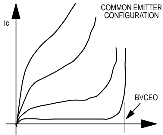
Figure 3b: At low impact ionization rate, the base current starts to increase, yielding an emitter current increase and, eventually, a collector current runaway
