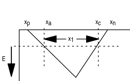
Figure 2a: Ionization occurs in the high field area x_1 of the space charge region
