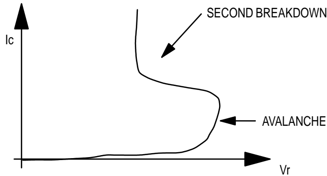
Figure 4. Typical Second Breakdown Characteristic
