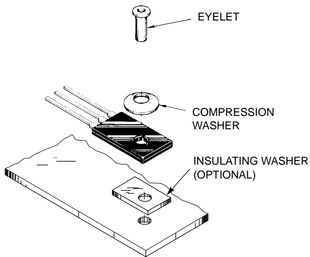
Figure 23. Eyelet Mounting
