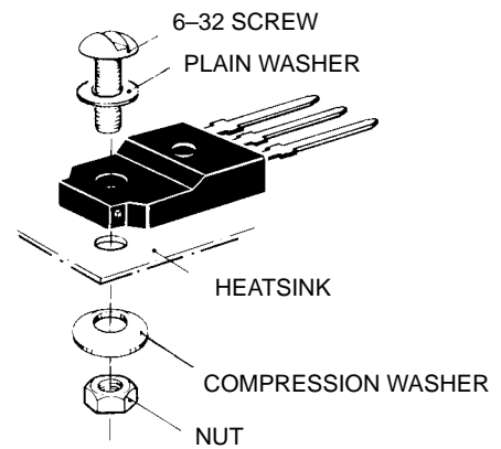
Figure 26. Screw-Mounted Isolated Package
