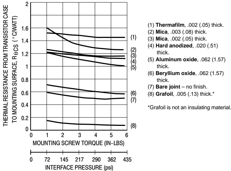
Figure 3. TO-204AA (TO-3) Without Thermal Grease
