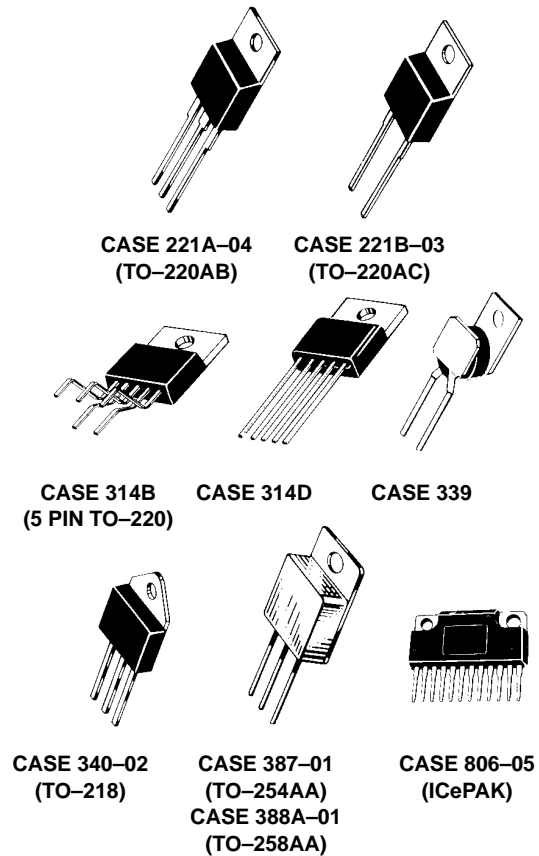
Figure 19. Several Types of Tab-Mount Parts
