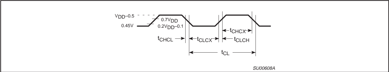
Figure 32. Clock Signal Waveform for I_{DD} Tests in Active and Idle Modes t_{CLCH} = t_{CHCL} = 5ns
