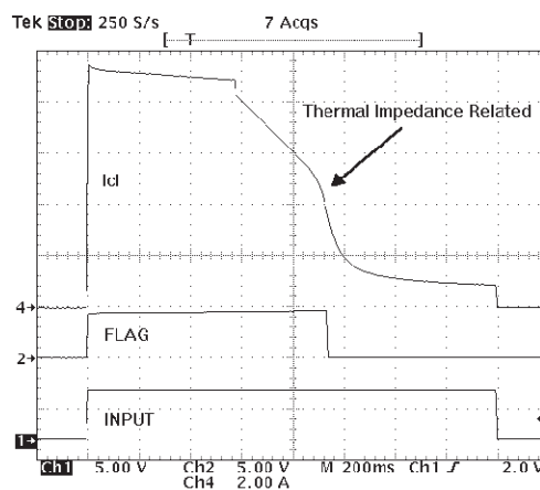
Fig. 2 Output Current Waveform After Thermal Protection Activation
