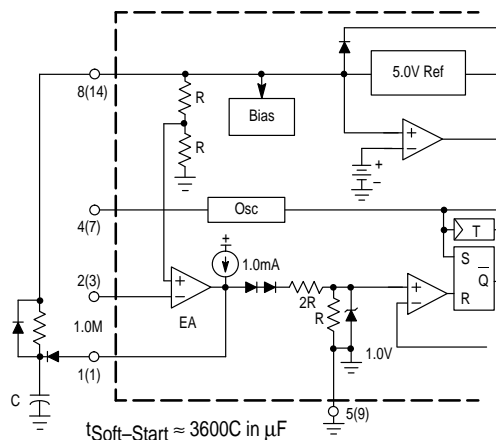
Figure 20. Soft-Start Circuit
