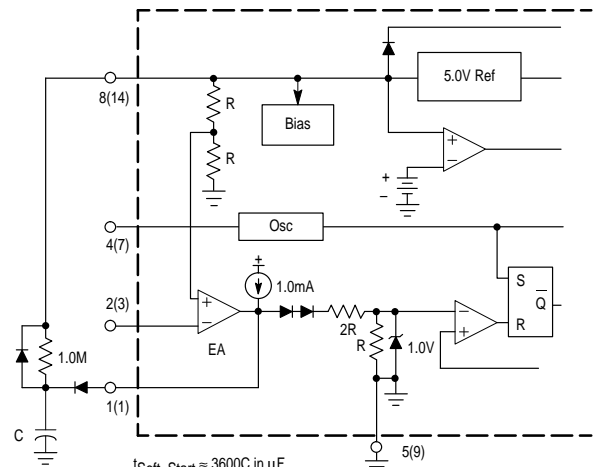
Figure 23. Soft-Start Circuit
