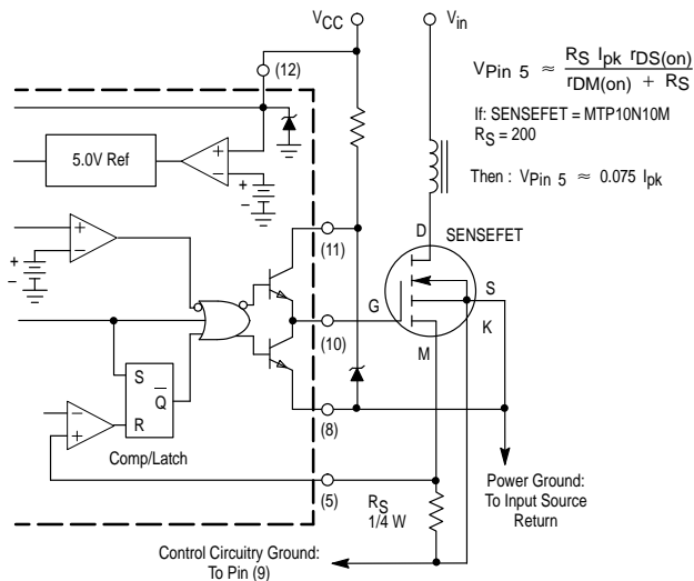
Figure 25. Current Sensing Power MOSFET
