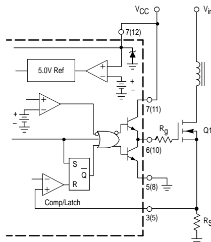
Figure 27. MOSFET Parasitic Oscillations
