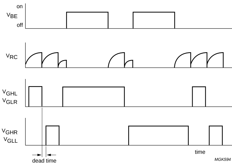
Fig.3 Timing diagram.
