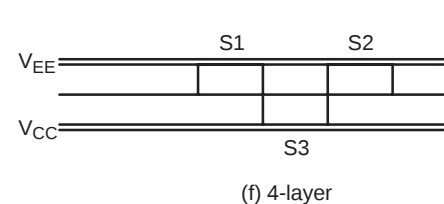
(f) 4-layer
