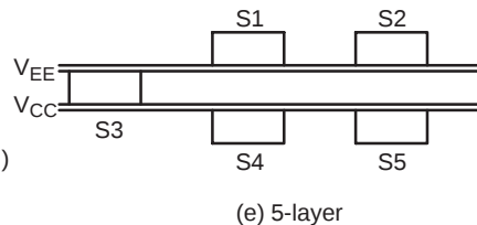
(e) 5-layer
