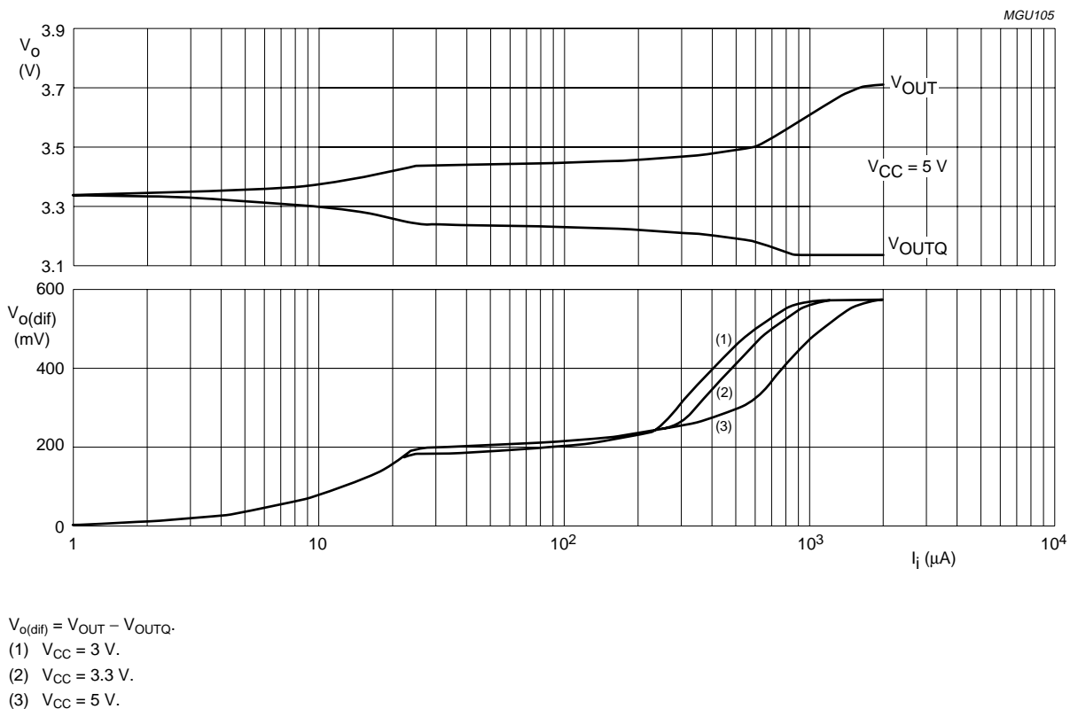
Fig.9 AGC characteristics.
