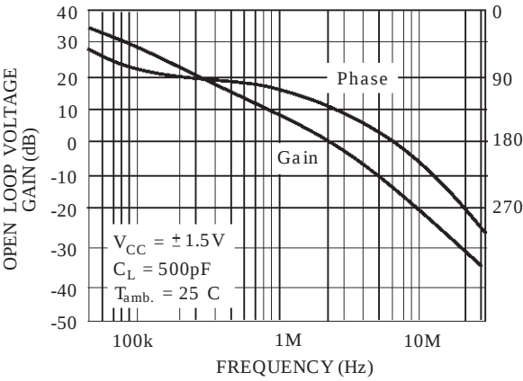
VOLTAGE GAIN AND PHASE VERSUS FREQUENCY
