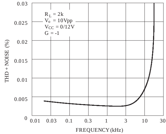
DISTORTION + NOISE VERSUS FREQUENCY
