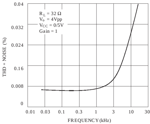
THD + NOISE VERSUS FREQUENCY
