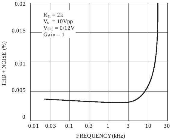
THD + NOISE VERSUS FREQUENCY
