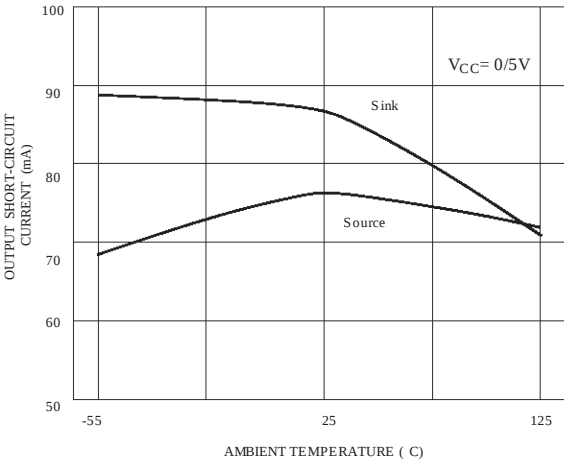
OUTPUT SHORT CIRCUIT CURRENT VERSUS TEMPERATURE
