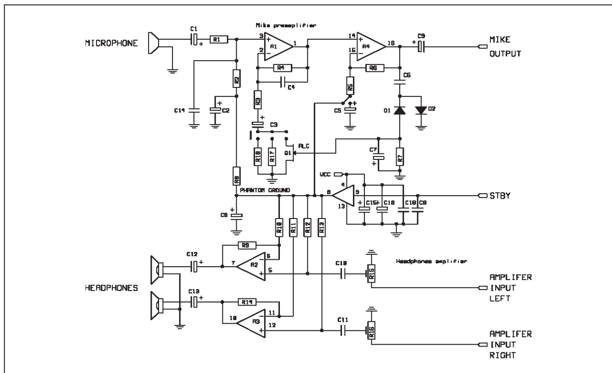
Figure 1 : Electrical Schematic
