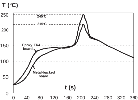
Fig. 10: Typical reflow soldering heat profile, either for mounting on FR4 or metal-backed boards.
