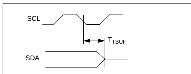
Figure 1-12. I 2 C I/O Timing
