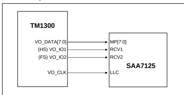
Figure 7-1. EVO connected to a digital video encoder (DENC).
