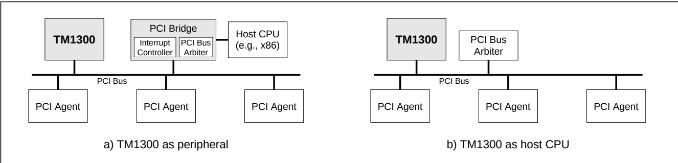
Figure 11-1. Two typical system implementations: (a) shows TM1300 as a PCI peripheral in a desktop PC, (b) shows an embedded system with TM1300 as the host CPU.
