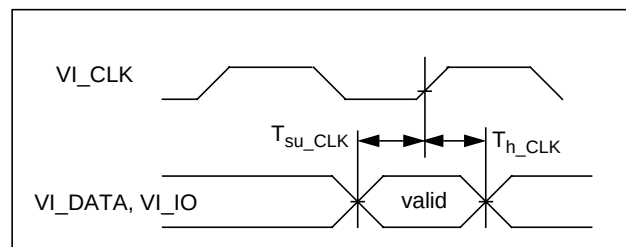
Figure 1-16. Video In I/O Timing
