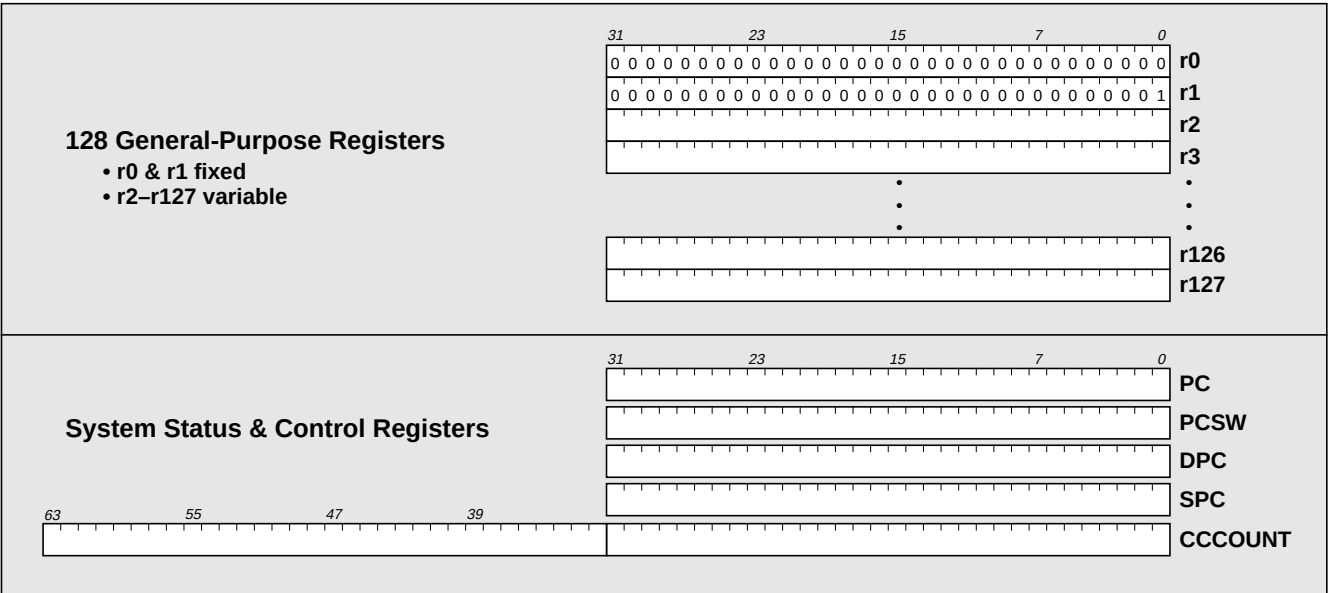
Figure 3-1. TM1300 registers.
