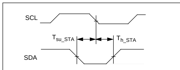
Figure 1-13. I 2 C I/O Timing
