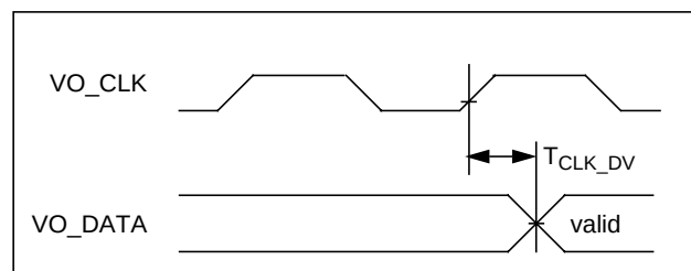
Figure 1-17. Video Out I/O Timing
