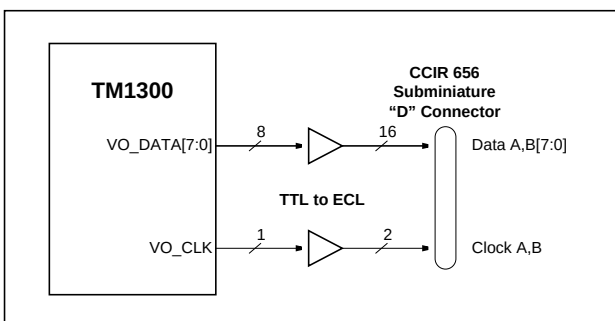
Figure 7-2. EVO connected to a CCIR 656 video-output connector.
