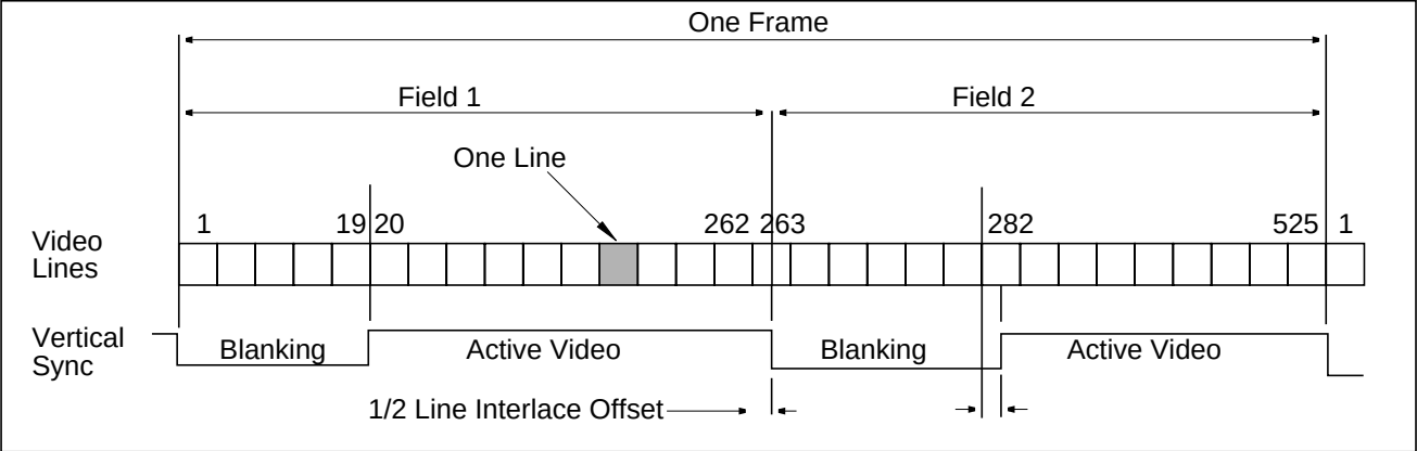
Figure 7-9. Interlaced timing—NTSC analog sync. signals.
