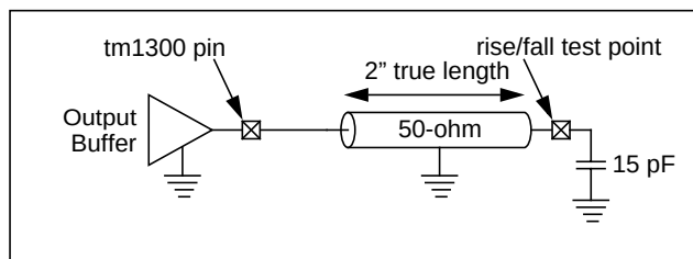
Figure 1-3. WEAK5 test load circuit
