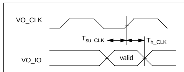
Figure 1-18. Video Out I/O Timing
