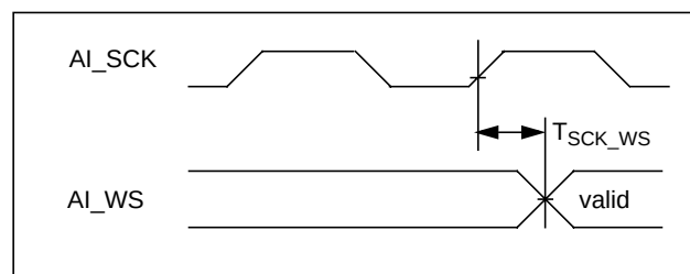
Figure 1-20. Audio In I/O Timing
