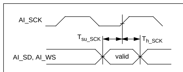
Figure 1-19. Audio In I/O Timing
