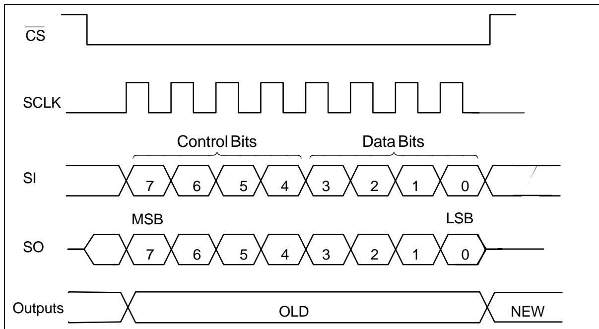
Figure 2: Serial Interface
