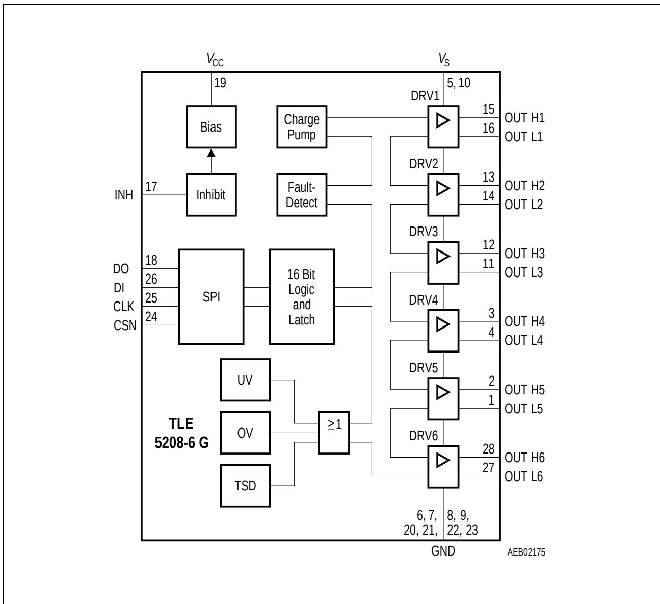
Figure 2 Block Diagram
