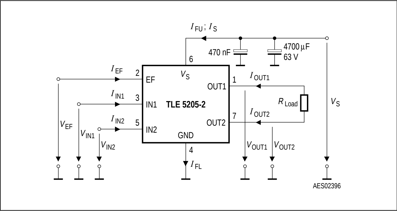
Figure 4 Test Circuit
