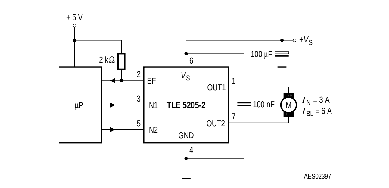
Figure 6 Application Circuit
