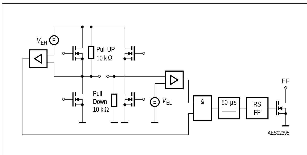
Figure 3 Simplified Schematic for Open Load Detection
