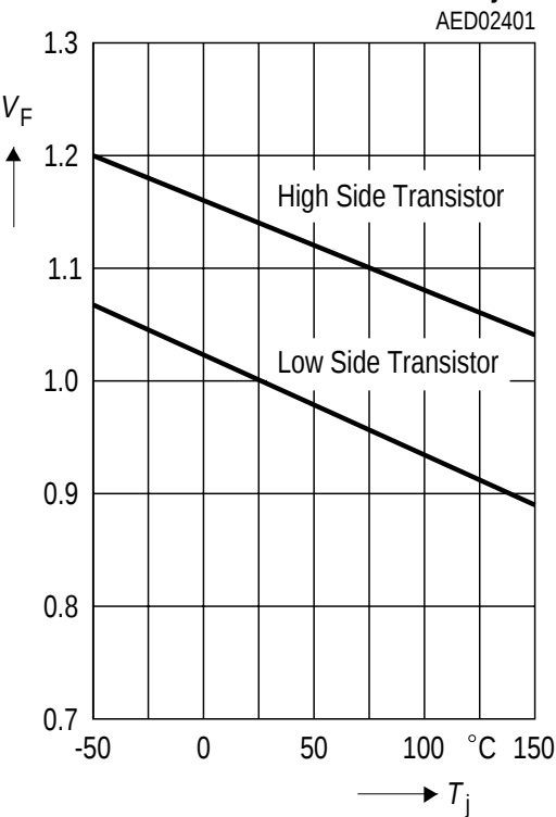
Clamp Diode Forward Voltage V_F versus Junction Temperature T_j
