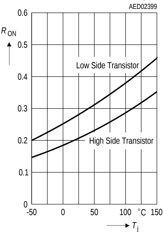
Static Drain-Source ON-Resistance versus Junction Temperature T_j
