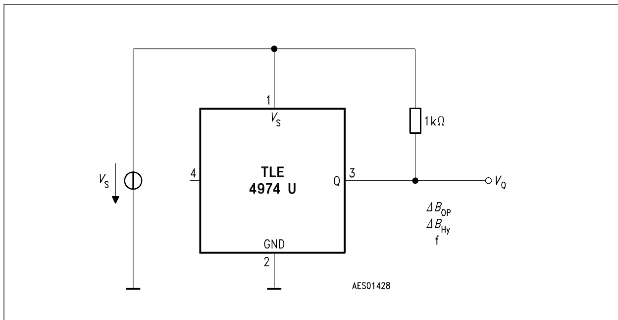
Figure 4 Test Circuit 2
