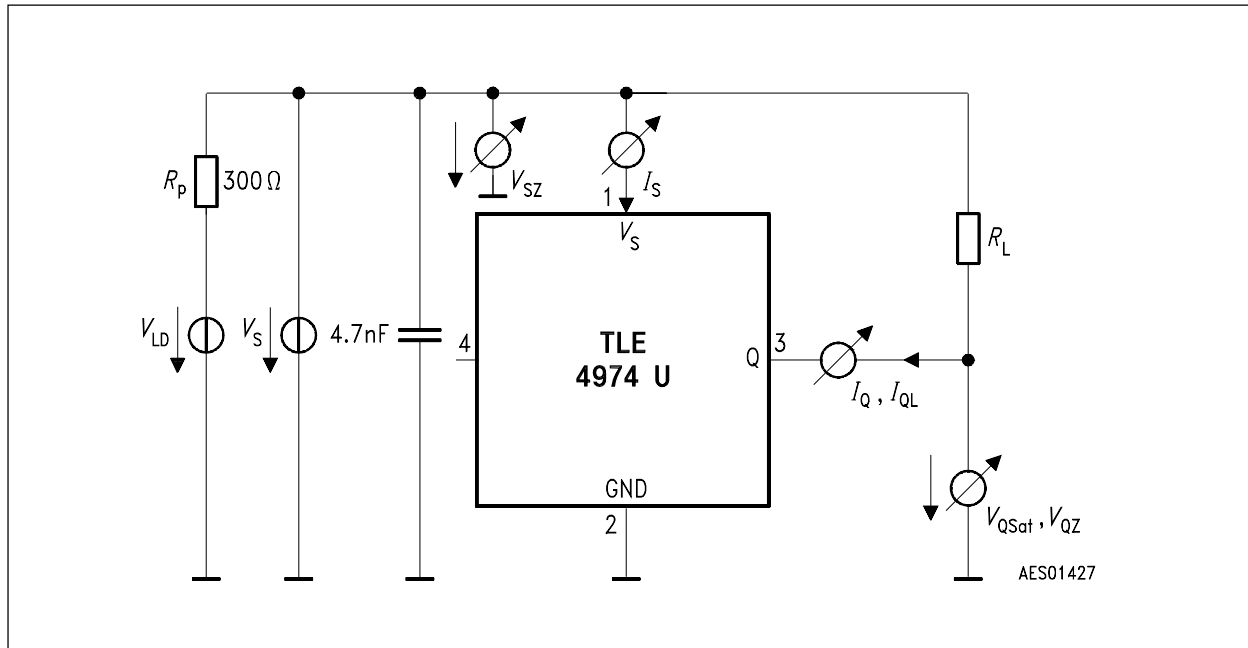
Figure 3 Test Circuit 1
