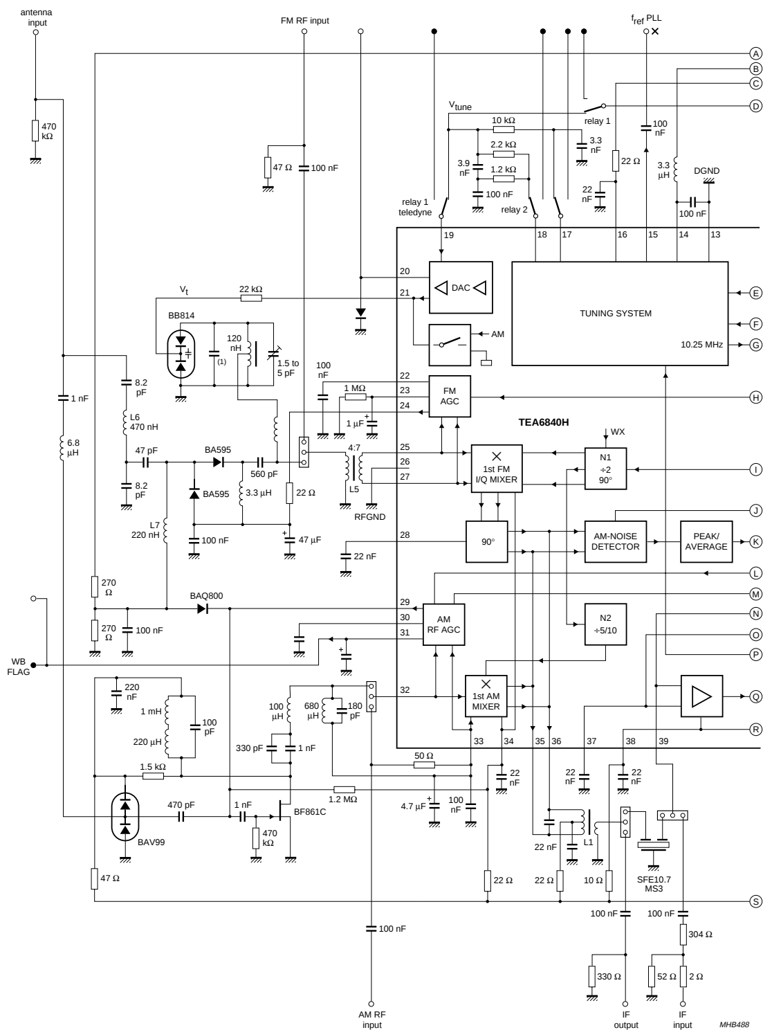
Fig.8 Test circuit (continued in Fig.9).
